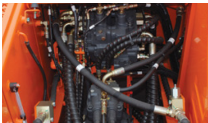
Swing drive
